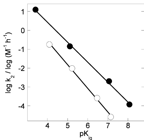
Fig. 3 Plot of k_2 versus pK_a of the leaving group for the reactions of S -aryl O -methyl phosphorothiolates (closed circles) and aryl methyl phosphates (open circles) with 3-picoline. The pK_a values 36,37 of the leaving groups for S -aryl O -methyl phosphorothiolates are: 2,4-dinitro, 3.2; 4-nitro, 5.11; 4-chloride, 7.06; and 4-methyl, 8.07. The pK_a values 32 of the leaving groups for aryl methyl phosphates are: 2,4-dinitro, 4.1; 2,5-dinitro, 5.22; 4-Cl-2-nitro, 6.46; and 4-nitro, 7.14.
